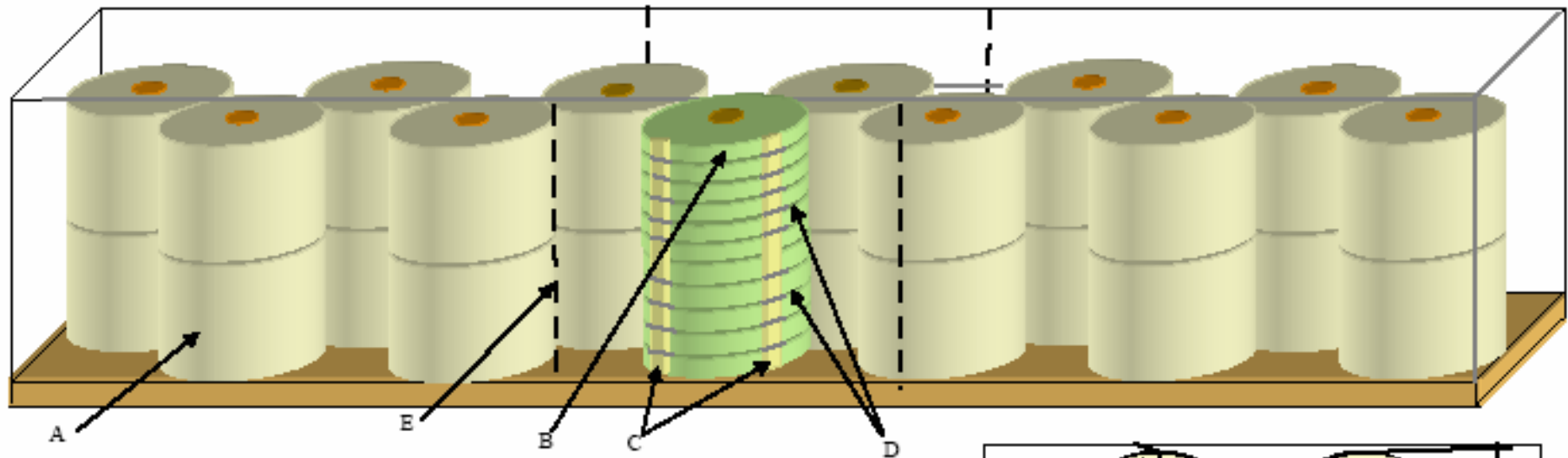
60 FOOT 8 INCH BY 9 FOOT 6 INCH BOX CAR LOADED WITH 72 INCH DIAMETER FIBER MAT.
